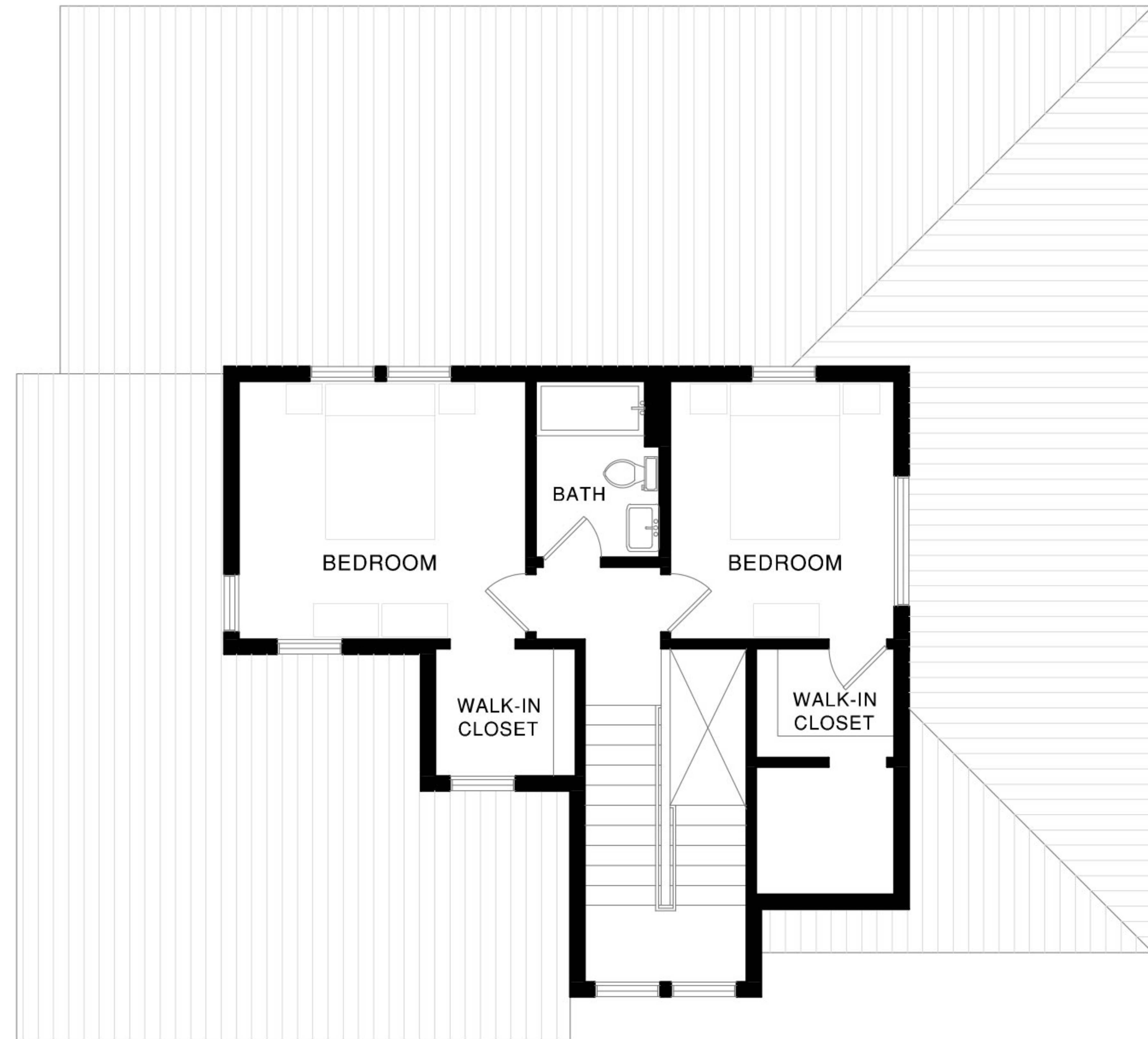
SECOND FLOOR
